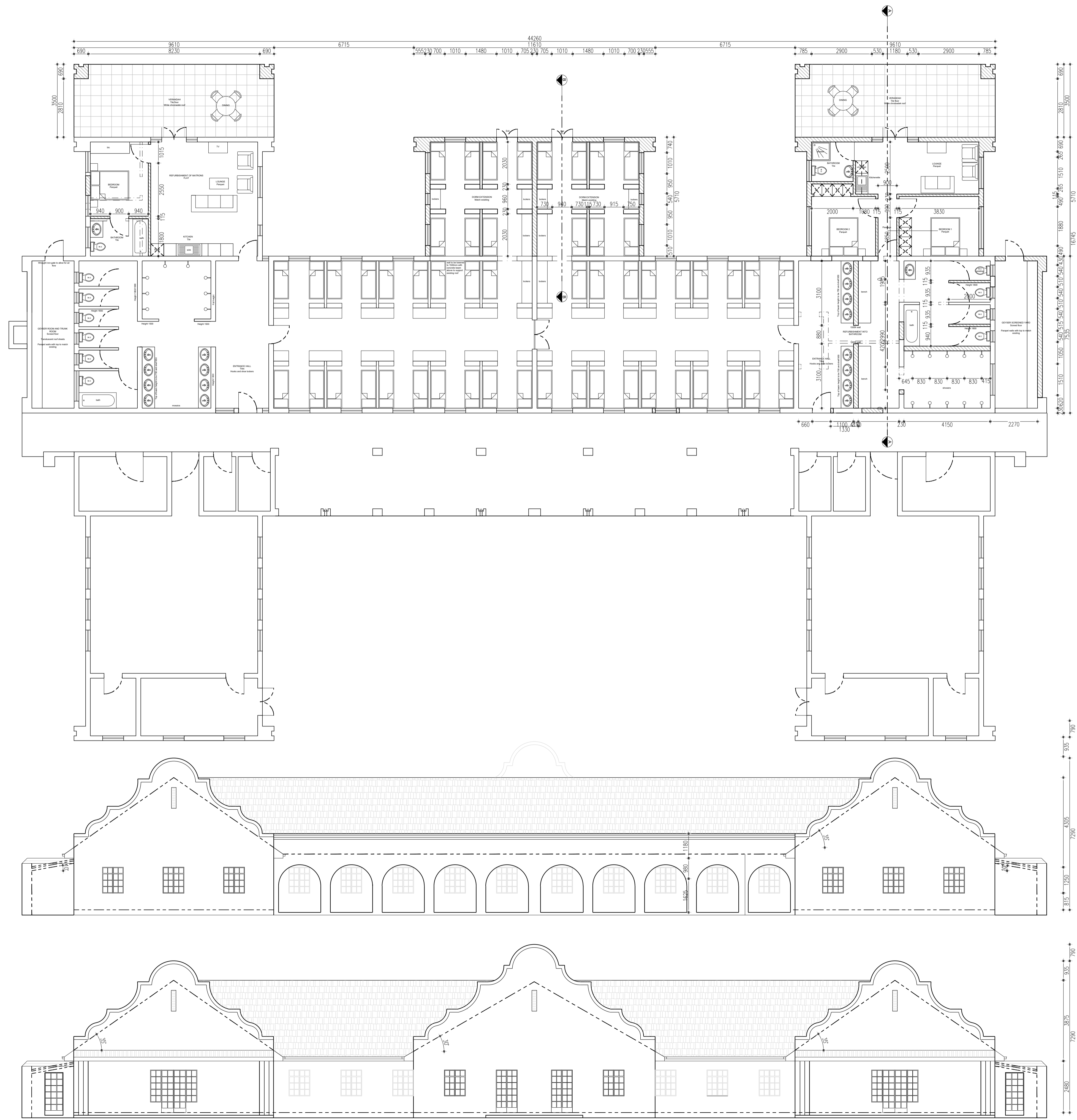
GROUND FLOOR PLAN SCALE- 1:100
